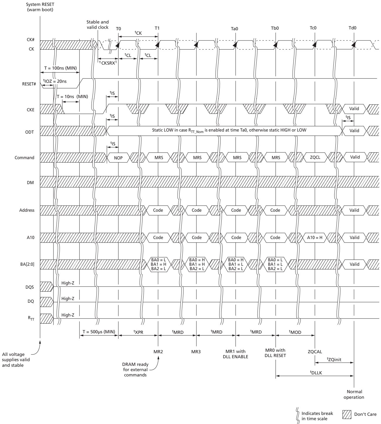
Figure 106: RESET Sequence
